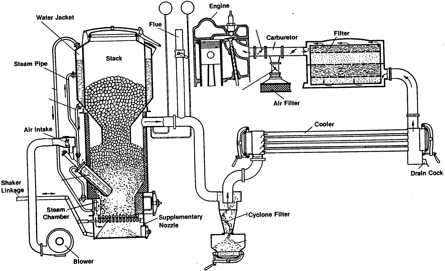
FIG. 43 PEGASUS OF HENSCHEL DESIGN
