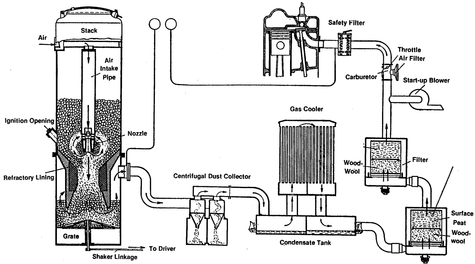
FIG. 44: PEGASUS OF ZEISSL DESIGN.
