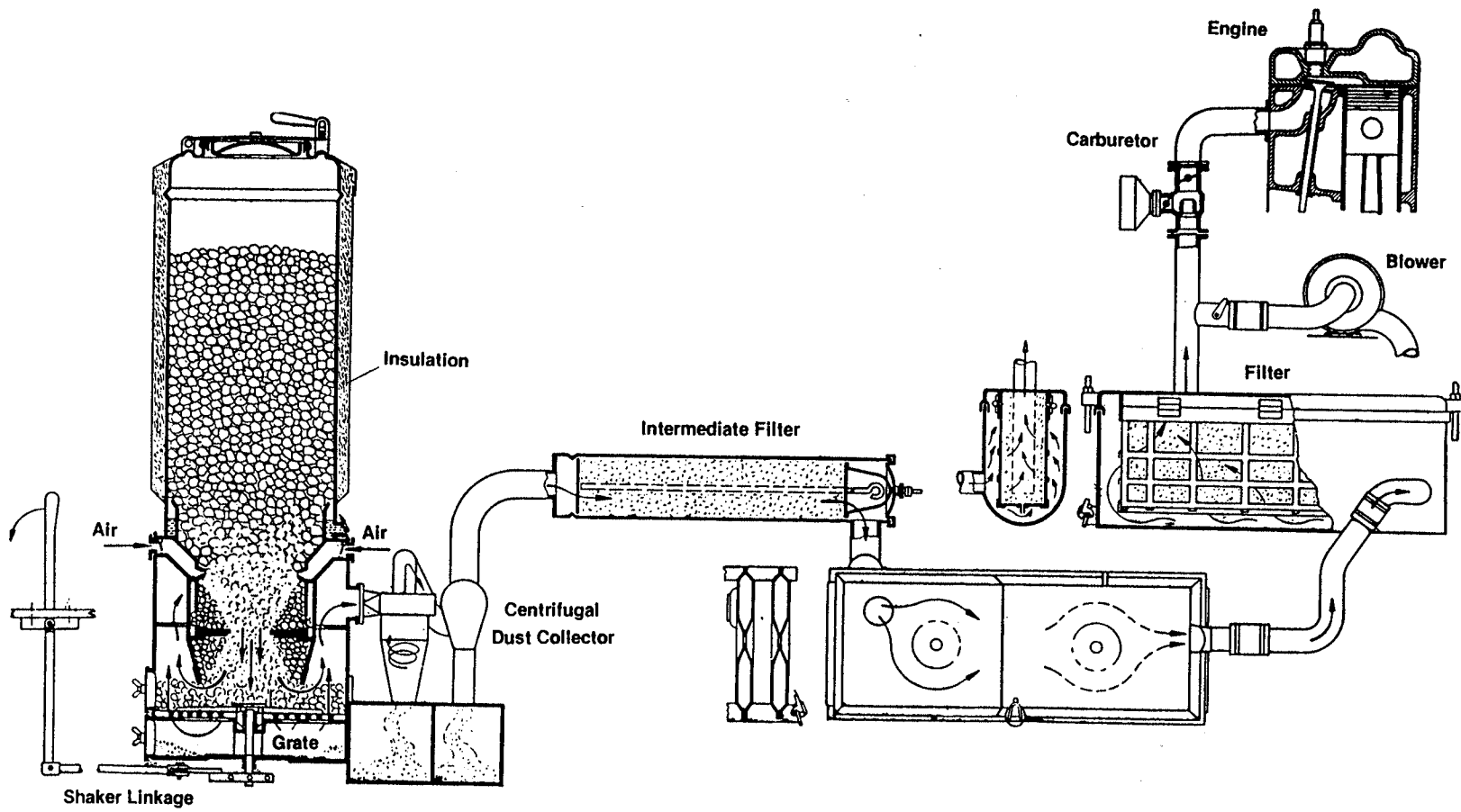
FIG. 46 PEGASUS OF ZEUCH DESIGN
