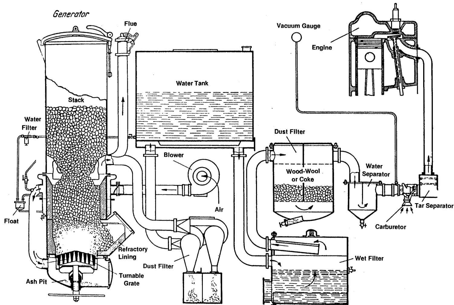
FIG. 49: PEGASUS OF STINNES DESIGN
