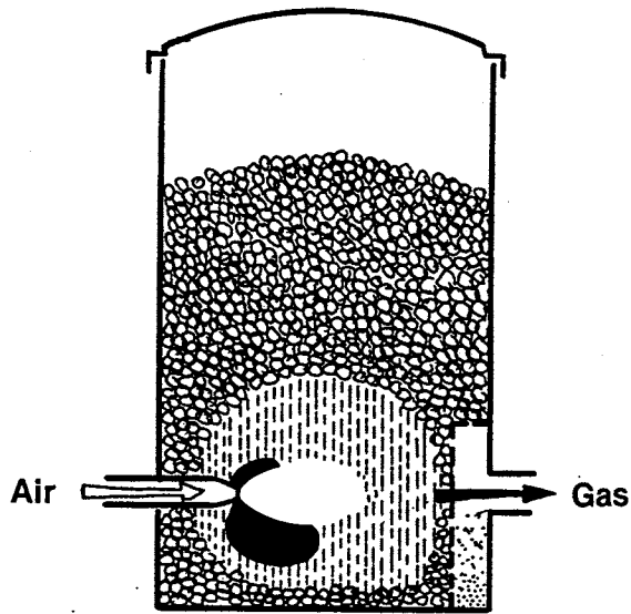
FIG. 17: CROSSDRAFT GASIFICATION
