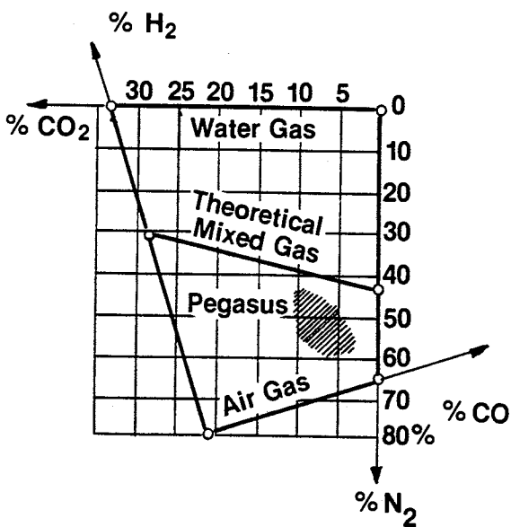
Fig. 5b Incombustible Constituents of the Pegasus Gas by Volume
