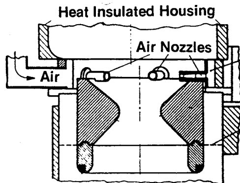
FIG. 30 CERAMIC HEARTH
