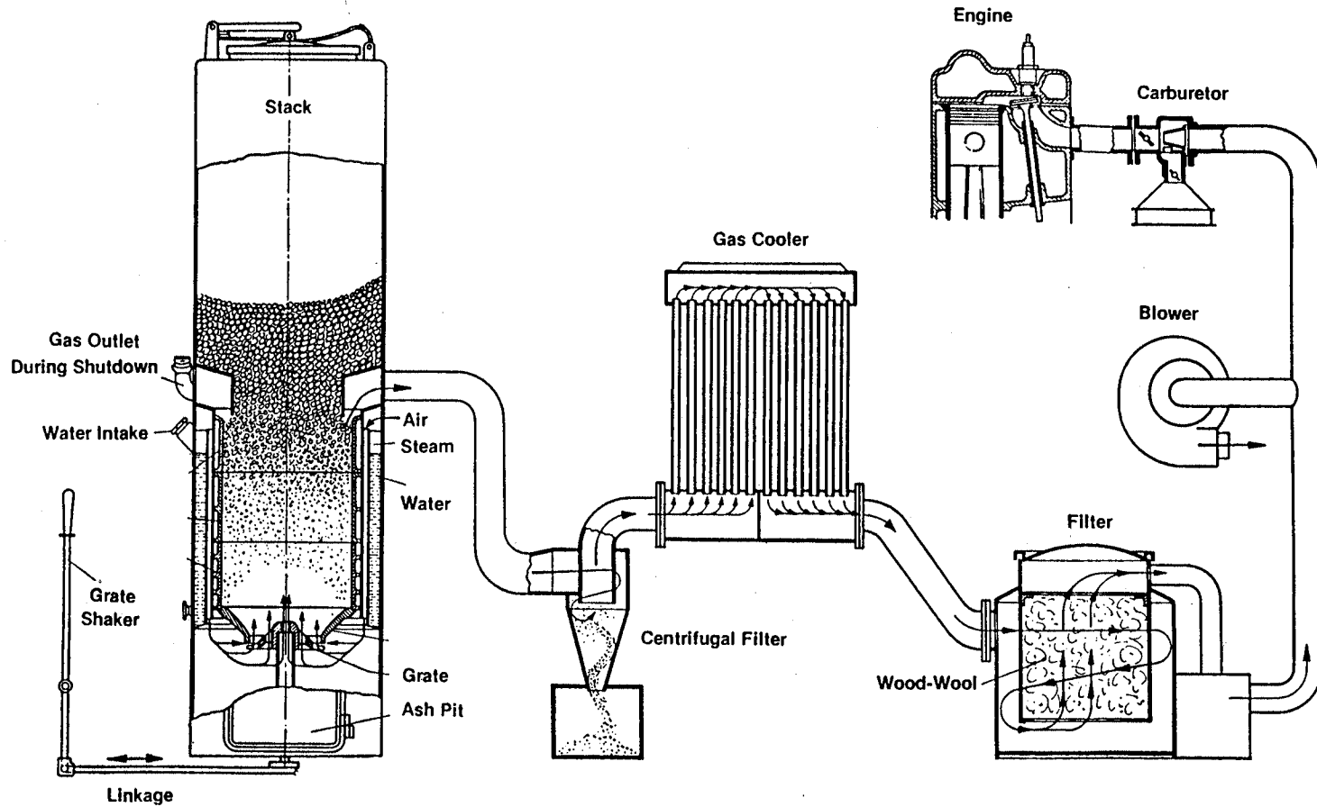
FIG. 45: PEGASUS OF GRUNERT DESIGN.
